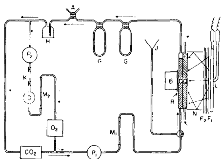
Fig. 1. Schematic diagram of apparatus for measuring quantum requirement of photosynthesis.
